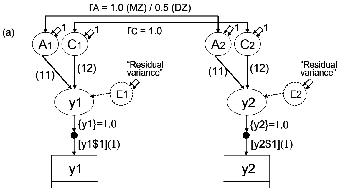
Figure 2. Mplus specification for a univariate twin model for a categorical variable. The phenotype is a binary variable, indicated by the rectangle with a single horizontal line. The binary variable is transformed into a continuous latent variable using a probit function based on the threshold and scaling factor.
