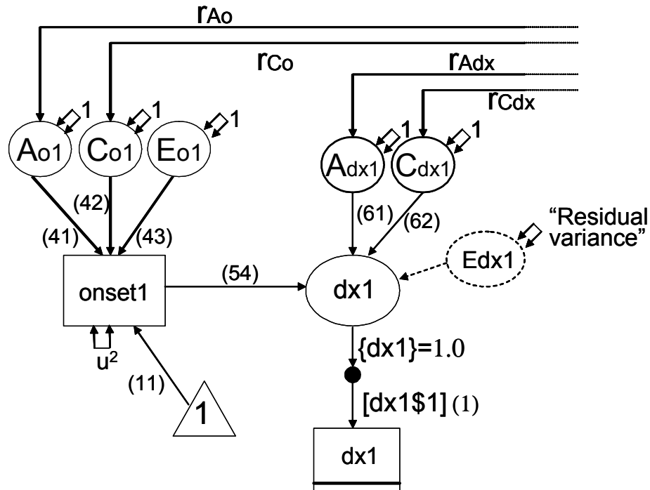
Figure 6. Mplus specification for a bivariate mediation model to test the hypothesis that onset directly mediates liability to diagnosis (Example 6). The model is shown for one individual (twin 1). Covariation between diagnosis liability and onset is modeled as occurring through onset. All sources of covariation (additive genetic, common environment and specific environment) in diagnosis liability occur in the same proportions as the sources of variation in the reliable portion of onset. A fixed estimate of onset unreliability ( u^2 ) is obtained from an external source.
