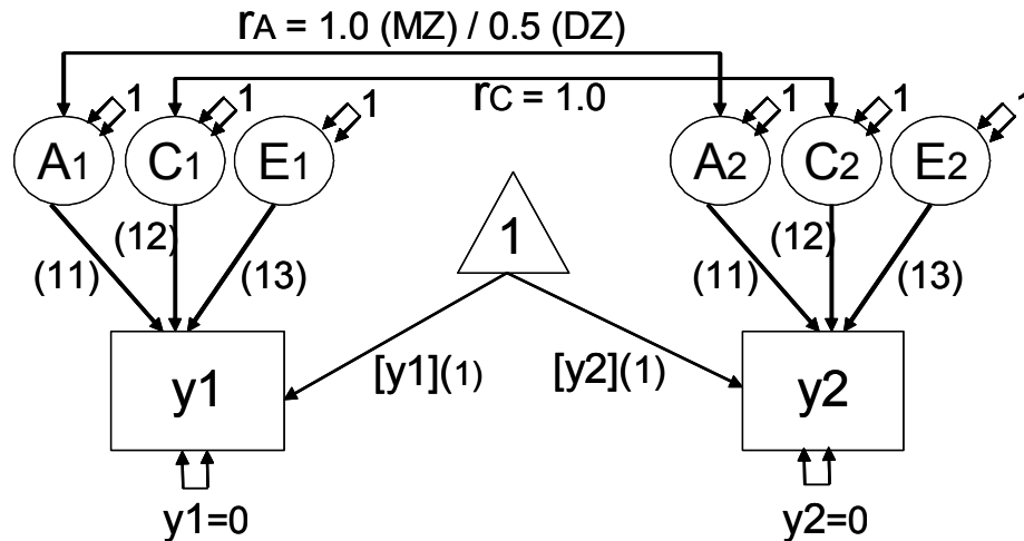
Figure 1. Univariate twin model for continuous variables as specified with the Mplus program. Numbers in parentheses correspond to the labels used for estimated parameters in the input script for Example 1. The estimated parameters include the observed variable intercepts ( [y_1] and [y_2] ), and three sources of variation. Residual variation for the observed scores is fixed to zero since this is confounded with E variation. Other fixed parameters include the latent variable variances (all fixed to 1) and the correlations between the genetic ( r_A ) and common environmental ( r_C ) latent variables
