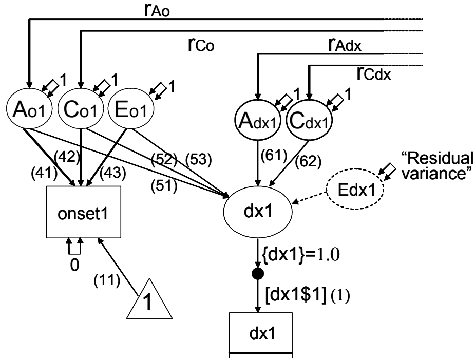
Figure 5. Mplus specification for a bivariate Cholesky decomposition model for estimating covariation between a continuous predictor variable and a binary outcome (Example 5). The model is shown for one individual (twin 1). One set of factors ( A_o, C_o, E_o ) contributes to variation in both onset age and liability to alcoholism diagnosis ( dx ). A set of residual factors contributes to the remaining variation in alcoholism liability. Individual-specific diagnosis residual variance is not estimated as an independent parameter, but is available as a calculated value in the Residual variance section of the program output.
