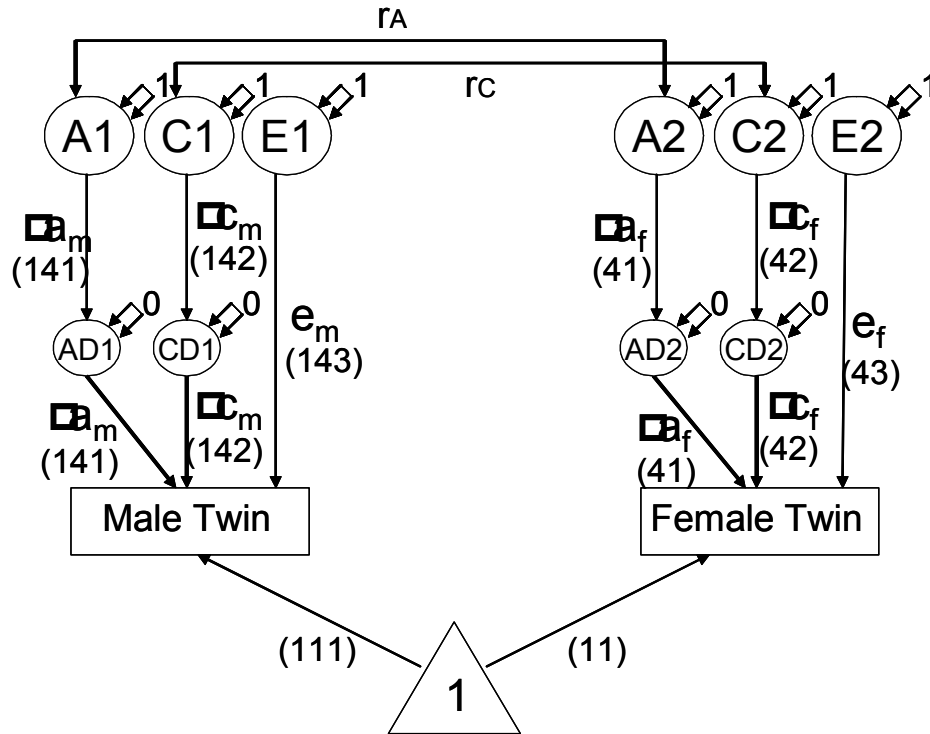
Figure 8. Mplus specification for a non-scalar sex differences model, parameterized to ensure male-female covariances are non-negative. Parameter labels correspond to the input script in Appendix VIII. The parameters as shown apply to opposite-sex pairs. This model uses placeholders to estimate the square roots of the additive genetic and common environment loadings.
